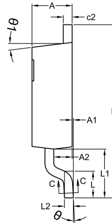
SIDE VIEW(Right)
